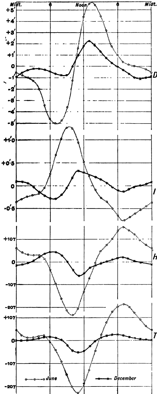
3.—KEW & QUIET DAY DIURNAL INEQUALITY.
